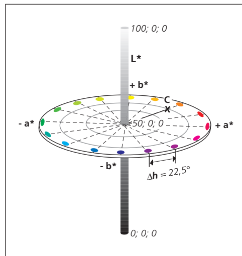
Diagram 3: the CIEL*a*b*-color space
